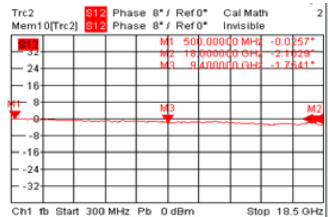
Phase Unbalance
