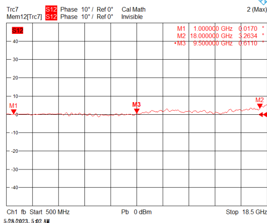
Phase Unbalance
