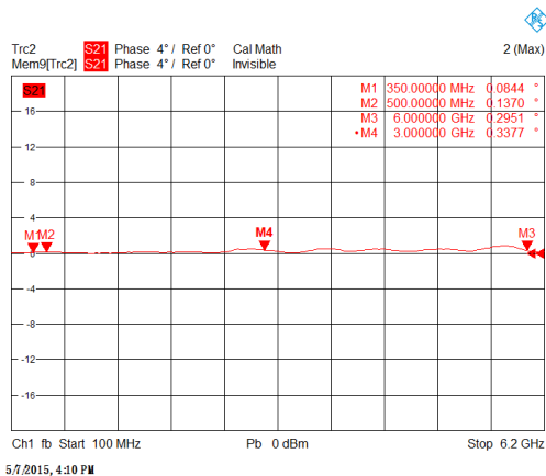
Phase Unbalance
